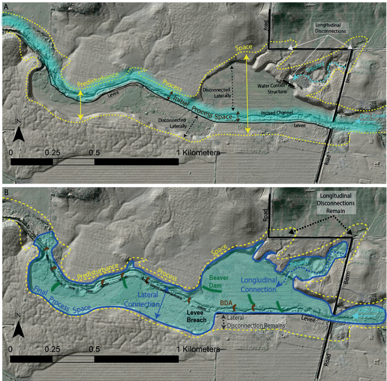
Figure 6. Process space limits are delineated for the Doty Ravine Creek Project to show (a) the total predisturbance space (outlined in yellow dashed line), prerestoration disconnected space, initially fluviually active space (highlighted blue), and (b) postrestoration final space (highlighted blue). Restoration actions that meet the space criteria result in a gain in process space for a project. This requires removing anthropogenic constrictions or modifying management to reconnect the floodplain (e.g., breach levees, repair road culverts, aggrade incised channel, beaver dam analogues (BDA) and control riparian grazing).
